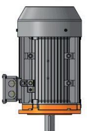
IMV18
